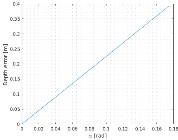
Figure 8.20: Plot of depth error vs. \alpha
