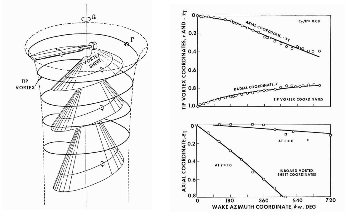
(a) Overview on propeller wake geometry. Both vortex sheet shedding from the propeller blade, and the tip vortex trajectory are shown. [25] (b) Measurements of the rotor wake shedding from double blade rotor [25]
