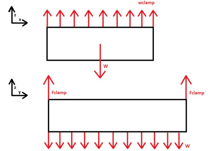
Figure 9.4: Free body diagrams of the payload box in the xz-plane and the zy-plan
