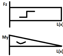
Figure 9.3: Shear force diagram above and the moment diagram below
