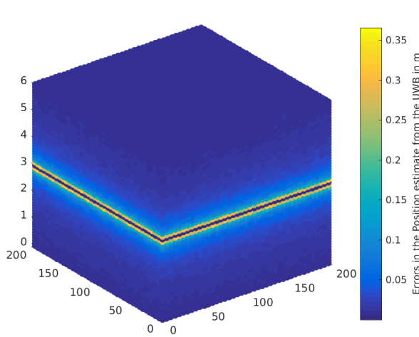
Figure 8.3: 3D plot of the accuracy of the UWB position estimates with tags placed at height of 3 m
