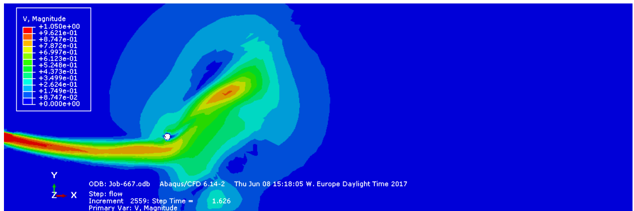
Figure 5.11: Flow on the cylinder: large eddy roll-up
