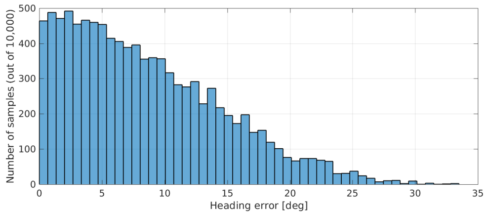
Figure 8.7: Histogram of the heading errors as observed from a simulation of 10,000 samples
