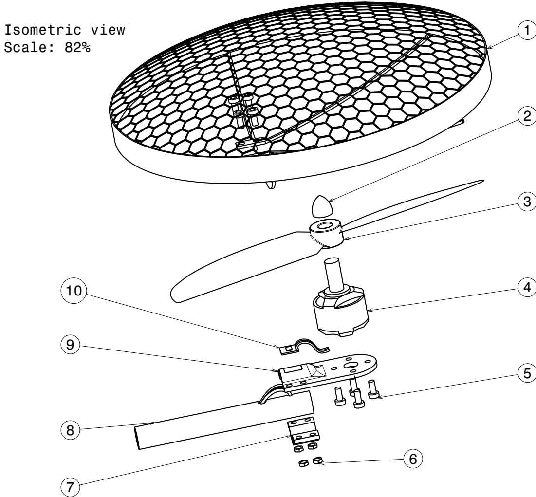
Figure 13.5: Exploded view of the propulsion assembly. Description of the balloon numbers is presented in Table 13.2
