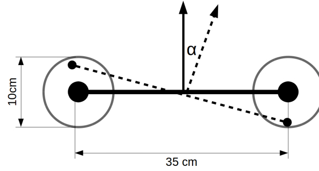
Figure 8.5: An illustration of the heading error estimation model. The big circles represent the actual UWB module locations while the smaller ones represent the position estimates. The spheres in which the positioning estimates can reside are also shown. The solid line is the true heading while the broken one is the estimated heading. The difference \alpha_e is the heading error
