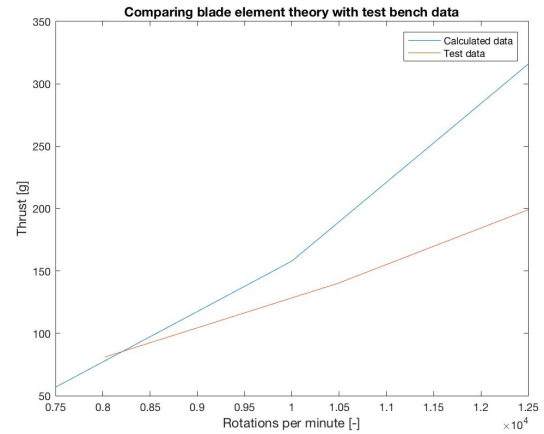
Figure 6.5: Comparing test data with blade element theory calculations
