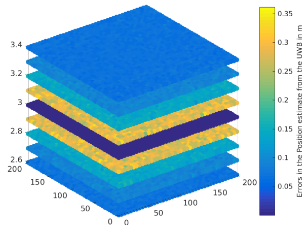
Figure 8.4: 3D plot of the accuracy of the UWB position estimates with tags placed at height of 3 m with zoom on the height close to height of the tags
